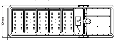
Dimension ( mm )
