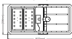
Dimension ( mm )
